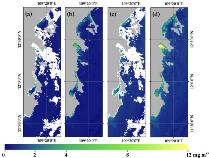
Figure 3.8. Illustration of DINEOF performance for the merged datasets in 2019: (a) original C2RCC, (b) filled C2RCC, (c) original DSF, (d) filled DSF
