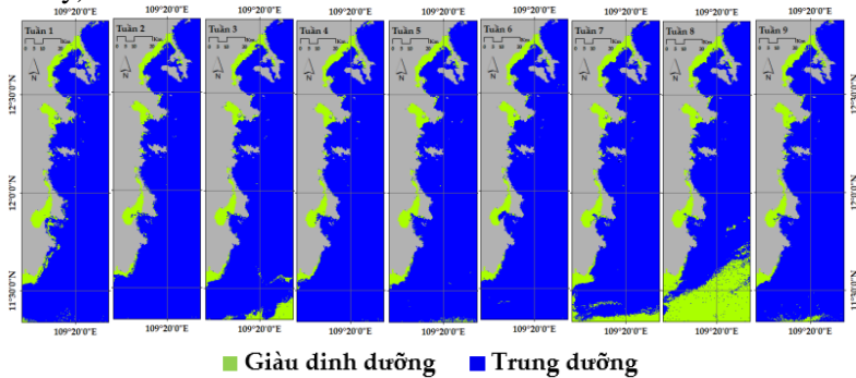
Figure 3.1. Weekly maps of eutrophic level from 01/07 to 31/08/2019
