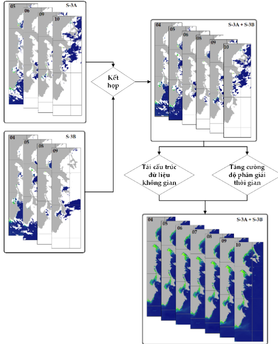
Figure 2.38. The solution handles spatial data affected by cloud cover and enhances temporal resolution when combining two satellites S-3A and S-3B, and the spatial data reconstruction model DINEOF.
