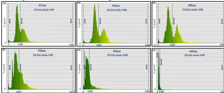
Figure 3.4. Histogram of water-leaving reflectance distribution in the wavelengths of 413nm, 443nm, 490nm, 510nm, 560nm, and 665nm
