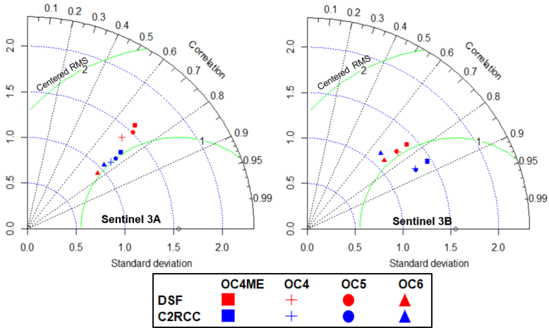
Figure 3.17. Taylor diagram represent the performance of different chl-a algorithms based on C2RCC and DSF, S-3A (left) and S-3B (right)
