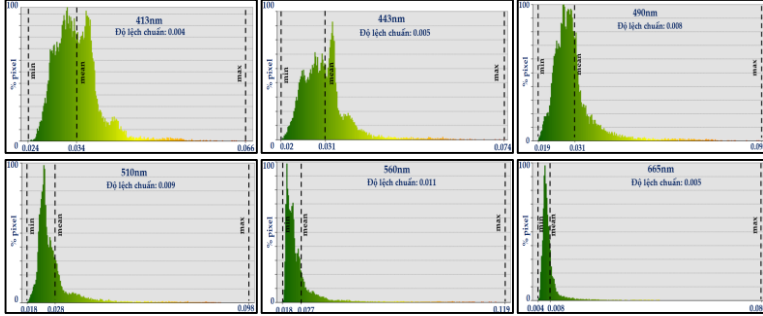
Figure 3.6. Histogram of water-leaving reflectance distribution in the wavelengths of 413nm, 443nm, 490nm, 510nm, 560nm, and 665nm over the research area. The atmospheric correction DSF (satellite S-3B, date of 05/07/2019)
