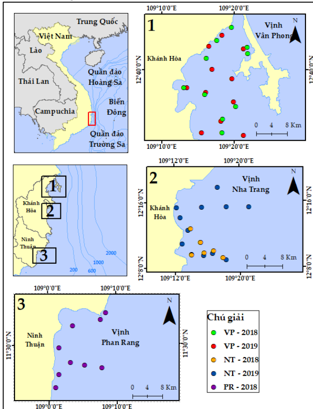
Figure 3.1. Location of the study area and field sampling
