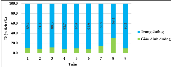
Figure 3.2. Statistics of eutrophic levels by percentage (%) over the study area. Pixels in oligotrophic were grouped to mesotrophic due to the negligible ( < 0,2\% )
