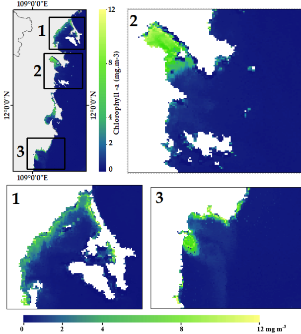
Figure 3.25. Synergy of both satellite S-3A and S-3B for Chl-a derived from OC5, July 31 st , 2019, Atmospheric correction C2RCC
