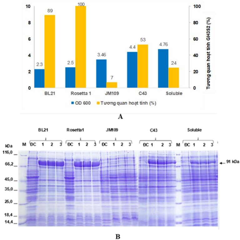
Figure 3.9. (A). Cell density and enzyme activity were obtained when expressed in expressed strains; (B). Electrophoresis of total GH3S2, DC: total protein of non-carrying vector control; 1, 2, 3: total protein of different lines 1, 2, 3 carrying the IPTG-inducible gh3s2 gene; M: standard protein (Fermentas)
