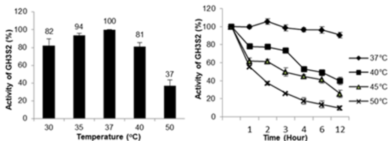
Figure 3.18. Effect of temperature on the activity and thermal stability of GH3S2 enzyme over time
