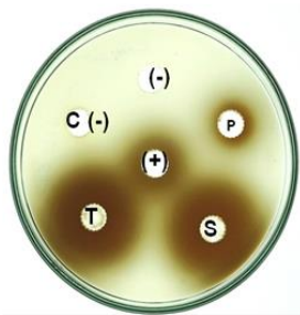
Figure 3.10. Check the activity of GH3S2 on LB agar plate using esculin substrate.
