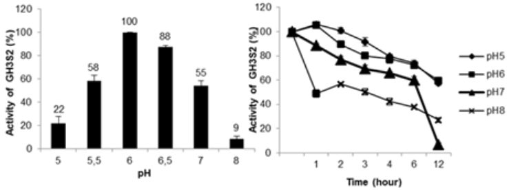
Figure 3.19. Effect of pH on the activity and pH stability of GH3S2 enzyme over time
