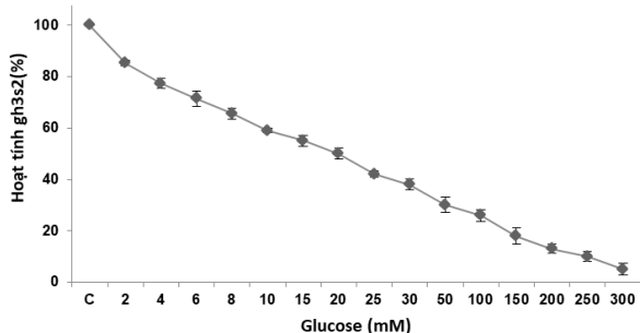
Figure 3.21. Effect of glucose on GH3S2 activity
