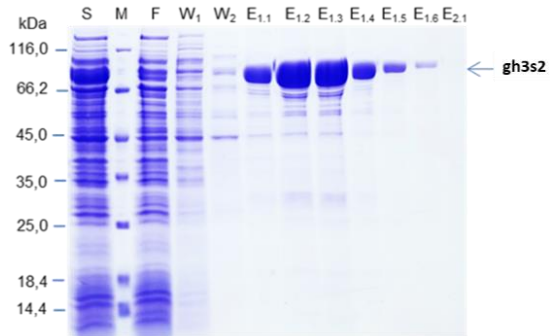
Figure 3.1. Electrophoresis of product in GH3S2 enzyme purification fractions on 12.5% polyacrylamide gel
