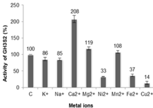
Figure 3.20. Effect of metal ions on GH3S2 activity
