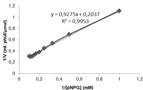
Figure 3.22. Reaction rate dependence of GH3S2 on pNPG substrate concentration according to Lineweaver – Burk
