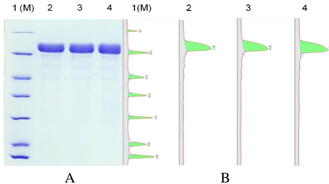
Figure 3.17. GH3S2 purity test results after purification (A). Electrophoresis of GH3S2 after purification (2 \mu g); (B). Cleanliness measurement results using Image Lab software
