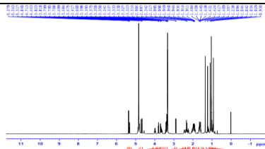
Figure 0.36. The ^1\text{H} NMR spectrum of SPI
