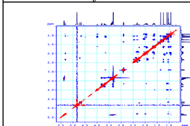
Figure 0.41. The NOESY spectrum and the important correlations of SPI
