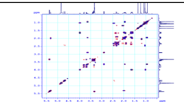
Figure 0.40. ^1\text{H} - ^1\text{H} COSY spectrum of SPI
