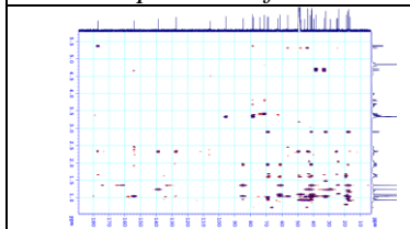
Figure 0.39. HMBC spectrum of SPI
