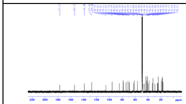
Figure 0.37. The ^{13}\text{C} NMR spectrum of SPI
