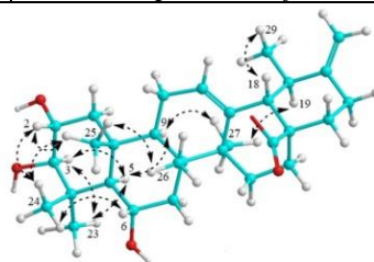
Figure 0.41. The NOESY spectrum and the important correlations of SPI
