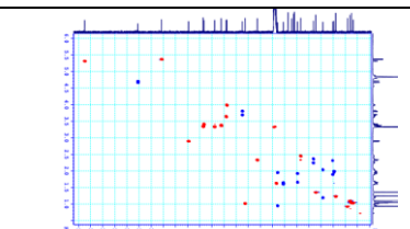
Figure 0.38. HSQC spectrum of SPI
