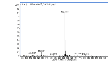
Figure 0.35. The (-)-HR-ESI-MS spectrum of SPI
