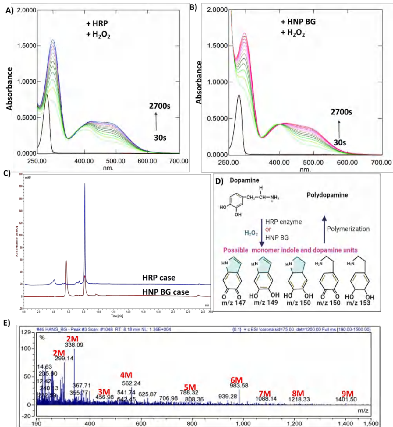
Figure 5.4: The oxidative pathway of DOPA under the catalyst of HRP enzyme or HNP BG in DI water.
