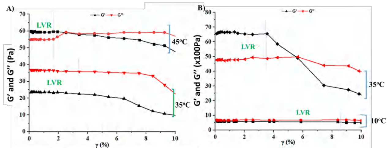
Figure 4.4: The viscoelastic parameters of two ACP copolymers (20 %wt) at different Pluronic contents.
