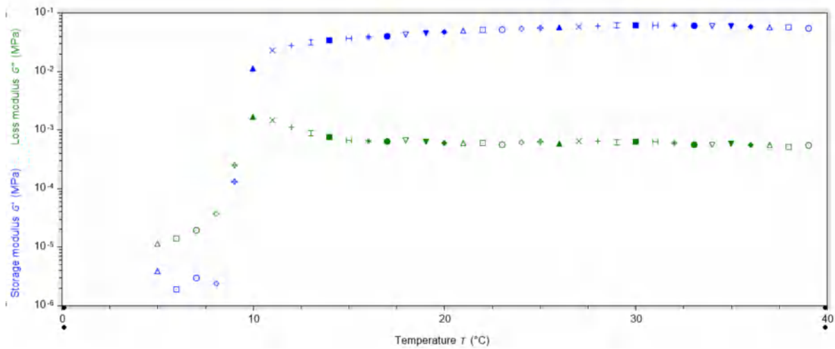
Figure A1: Temperature sweep function of pure Pluronic F127 at 20 wt%.
