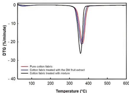
Figure 3.22. DrTG diagrams of antibacterial-treated cotton fabric samples
