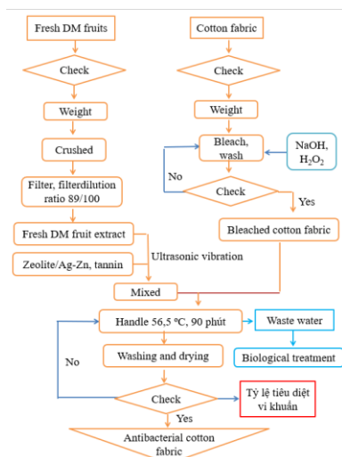
Figure 3.11. Procedure for treatment of cotton fabric with the optimal mixture
