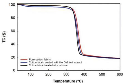
Figure 3.21. TG diagrams of antibacterial-treated cotton fabric samples
