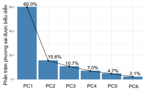
Figure 4.6. Variance drop plot of principal components
