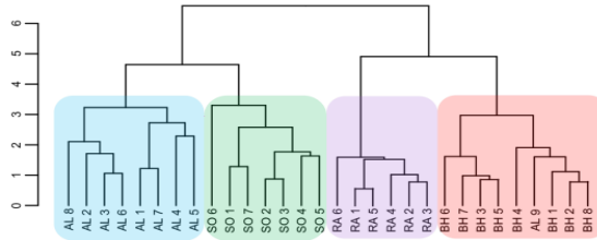
Figure 4.5. Tree diagram of Atractylodes macrocephala based on quantified metabolite content.
