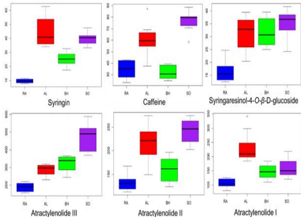
Figure 4.8. Box plot of reference substance content in Atractylodes macrocephala sample groups
