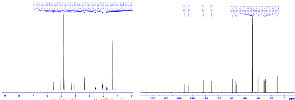
Figure 4.2. ^1\text{H} NMR and ^{13}\text{C} NMR spectrum of compound AMI
