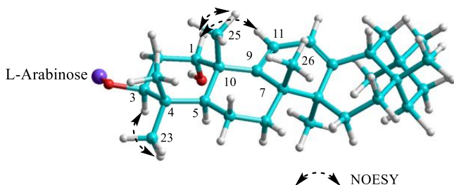
Figure 4.12. Key NOESY correlations of MS1
