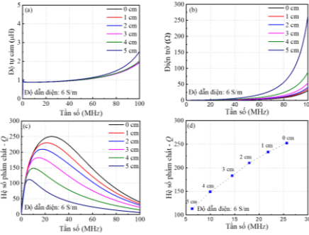
Figure 3.5. Dependence of the parameters of the resonant coil on frequency at different thicknesses of the conductor block: (a) inductance, (b) resistance, (c) quality factor and (d) maximum quality factor.
