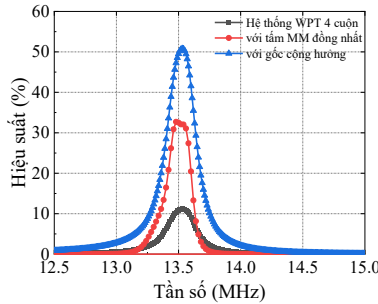
Figure 4.8. Measured performance of the MR-WPT system in the following cases: without MM slab (4-coils MR-WPT system), with homogeneous MM slab, and with MM slab with resonant cavity.
