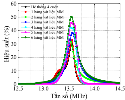
Figure 3.17. Measurement performance of the original MR-WPT system and when using the rollable MM slab with each row of MM unit cells as illustrated in Figure 3.13 at the transmission distance d_{\text{Tx-Rx}} = 250 mm.
