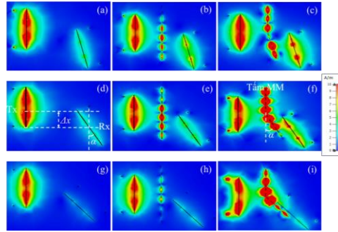
Figure 3.15. Simulation results of magnetic field distribution in MR-WPT system when Rx is offset \Delta x = 100 mm and the angular deviation is 15^\circ , 30^\circ , 45^\circ respectively in the following cases: (a), (d), (g) when the system without MM slab; (b), (e), (h) when the system with a straight MM slab; (c), (f), (i) when the system has a MM slab folded at an angle corresponding to the deviation angle of Rx.
