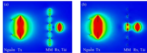
Figure 4.5. Simulation results of magnetic field distribution in MR-WPT system: (a) with homogeneous MM, (b) with non-homogeneous MM slab.
