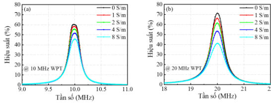
Figure 3.7. Measured performance dependence on operating frequency of MR-WPT systems with different conductivities: (a) MR-WPT operating at 10 MHz range, (b) MR-WPT operating at 20 MHz range.
