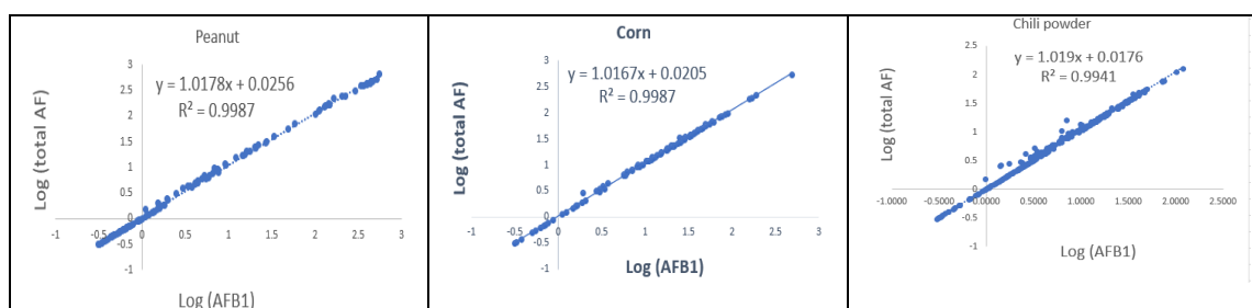
Figure 3.17: Correlation between AFB1 contamination content and total AF for peanut, chili powder, and corn
