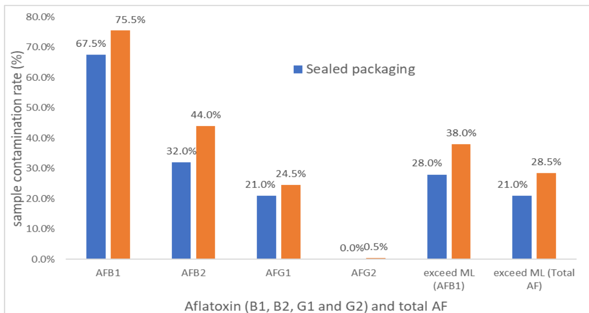
Figure 3.13: Comparison chart of the percentage of AFB1 contaminated samples, exceeding the allowable AFB1 level, total AF in sealed (blue) and unsealed (orange) packaging
