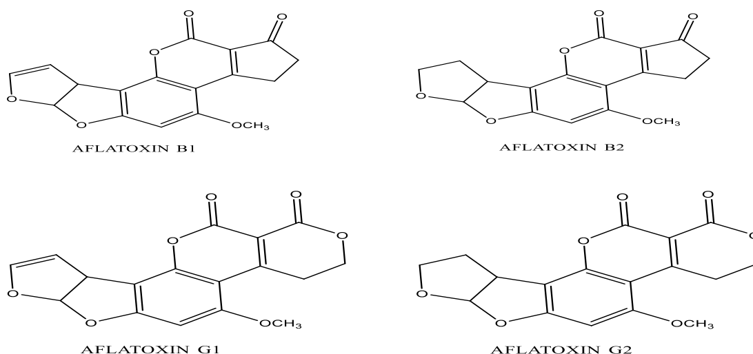
Figure 1.1: Molecular structure of the four main types of aflatoxins
