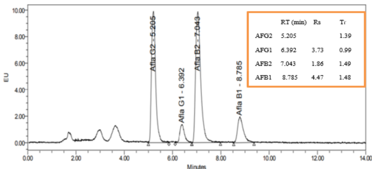
Hình 3.1: Standard chromatogram 10 µg/L in ACN/0.2% HCOOH with mobile phase composition 0.1% HCOOH/ACN/MeOH (64/18/18)
