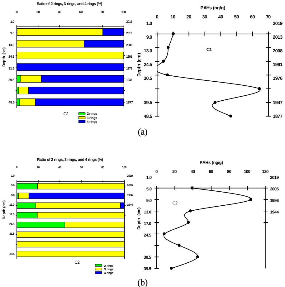
Figure 3.17. Distribution of PAHs in the sediment cores
