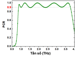
Figure 4.22. Absorption efficiency and polarization conversion efficiency
