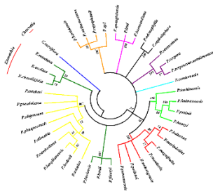
Figure 1. Phylogenetic tree based on morphological characters of species belonging to the genera Psychotria , Eumachia , and Chassalia in Vietnam.
