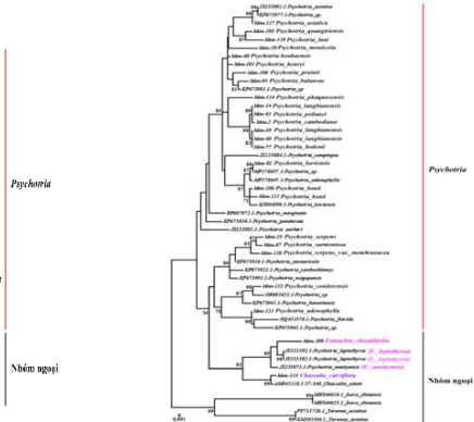
Figure 4. Phylogenetic tree constructed for species in the genus Psychotria based on ITS2 sequences.
