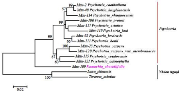
Figure 5. Phylogenetic tree of Psychotria species constructed based on combined matK and ITS2 sequence data.
