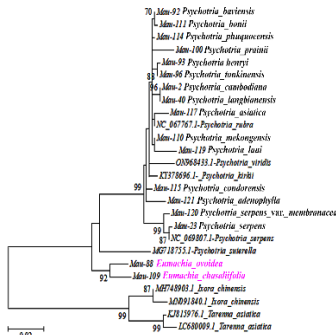
Figure 3. Phylogenetic tree constructed for species in the genus Psychotria based on matK sequences.
