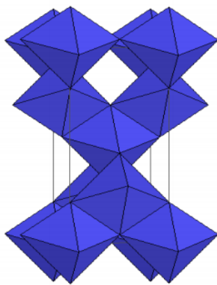
Anatase
