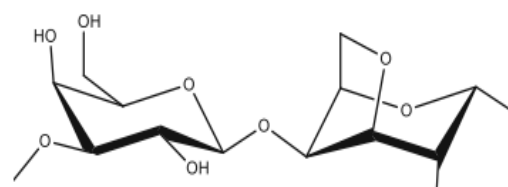
\delta -carrageenan G - D2,6S
