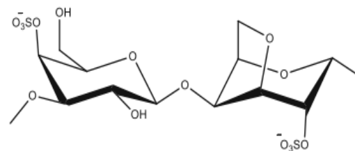
\iota -carrageenan 3-linked \beta -D-galactopyranose-4-sulfate (G4S) 4-linked 3,6-anhydro- \alpha -D-galactopyranose-2-sulfate (DA2S)
