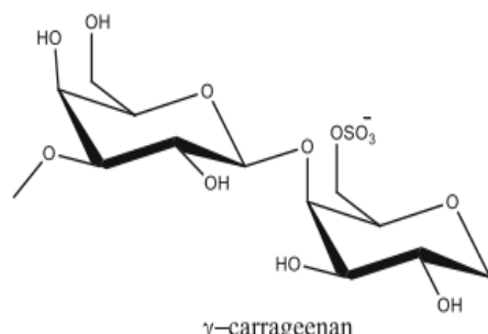
\gamma -carrageenan 3-linked \beta -D-galactopyranose (G) 4-linked \alpha -D-galactopyranose-6-sulfate (D6S)
