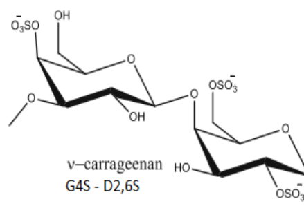
\iota -carrageenan 3-linked \beta -D-galactopyranose-4-sulfate (G4S) 4-linked 3,6-anhydro- \alpha -D-galactopyranose-2-sulfate (DA2S)
