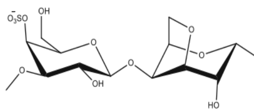
\kappa -carrageenan 3-linked \beta -D-galactopyranose-4-sulfate (G4S) 4-linked 3,6-anhydro- \alpha -D-galactopyranose (DA)
