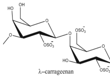
\nu -carrageenan G4S - D2,6S
