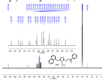
Figure 3.11. ^{13}\text{C} -NMR spectrum of compound H 1
