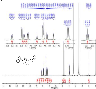
Figure 3.10. ^1\text{H-NMR} spectrum of compound K 1
