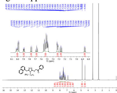
Figure 3.9. ^1\text{H-NMR} spectrum of compound H 1
