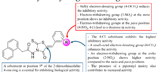
Figure 3.3. Structure–activity relationship of compounds E 1-11
