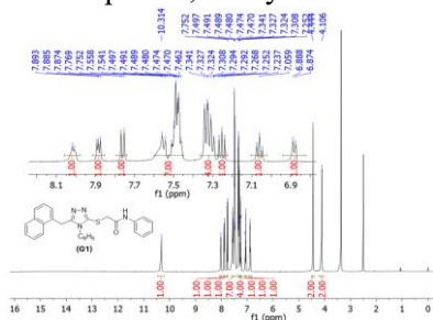
Figure 3.5. 1 H-NMR spectrum of compound G 1
