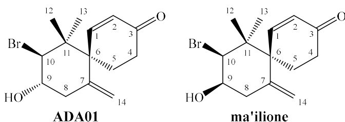
Fig. 3.1. Structure of ADA1
