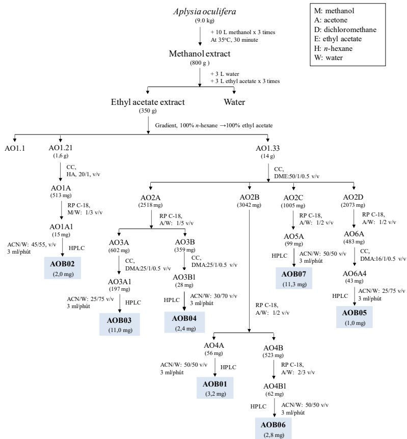
Fig. 2.7. Diagram of isolation of compounds from A. oculifera
