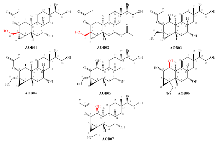
Fig. 3.3. Structure of compounds AOB1 - AOB7 from A. oculifera
