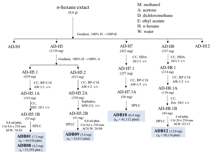
Fig. 2.5. Diagram of isolation of compounds from n -hexane of A. dactylomela
