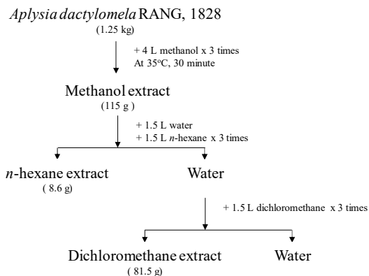
Fig. 2.4. Diagram of isolation of compounds form A. dactylomela in Quang Ngai
