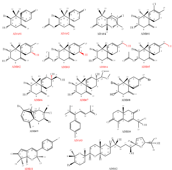
Fig. 3.2. Structure of compounds from A. dactylomela
