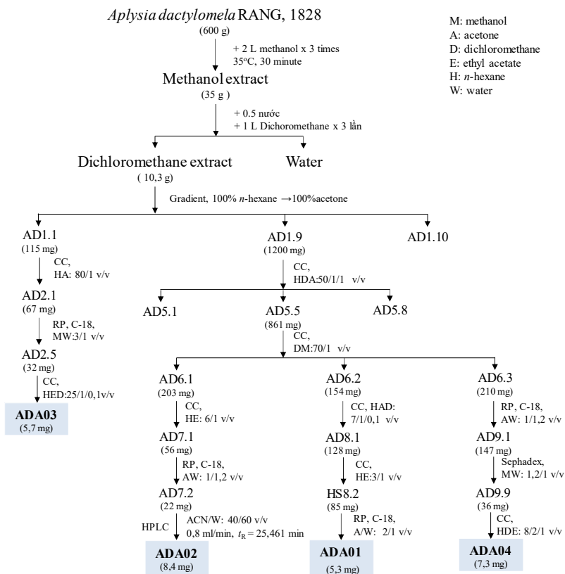
Fig. 2.3. Diagram of isolation of compounds from A. dactylomela
