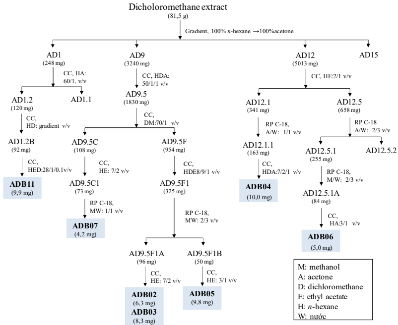
Fig. 2. 6. Diagram of isolation of compounds from dichloromethane extract of A. dactylomela
