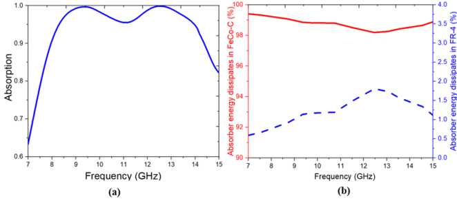
Figure 3.6. Absorption spectrum of the designed CM-MA structure and (b) the captured energy dissipated in the FeCo-C and FR-4 layer in the CM-MA structure.
