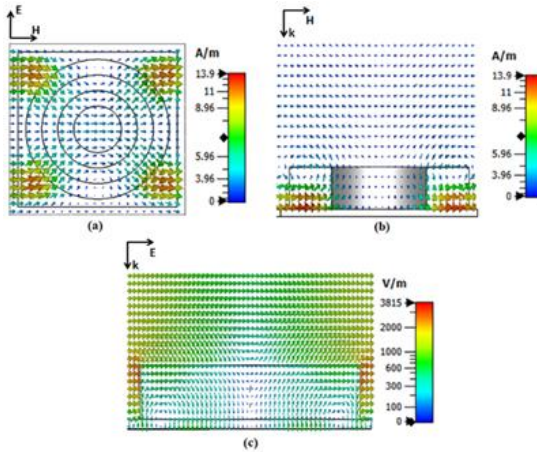
Figure 3.7. Electric- and magnetic-field distribution of the CM-MA structure. (a) Magnetic field in the (E, H) plane, (b) magnetic field in the (H, \mathbf{k}) plane and (c) electric field in the (E, \mathbf{k}) plane at a frequency of 9.4 GHz.
