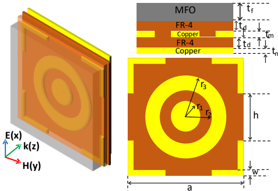
Figure 4.16. Schematic of CM-MA based MFO unit cell.
