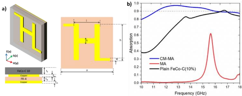
Figure 3.31. (a) Schematic of CM-MA based FeCo-C (10%) unit cell, (b) Comparison of absorption spectra for plain FeCo-C(10%), MA and CM-MA.
