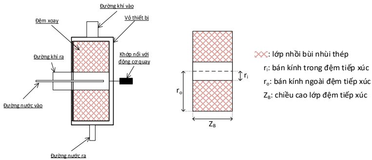
Figure 2.1. Structure of the HP2R device
