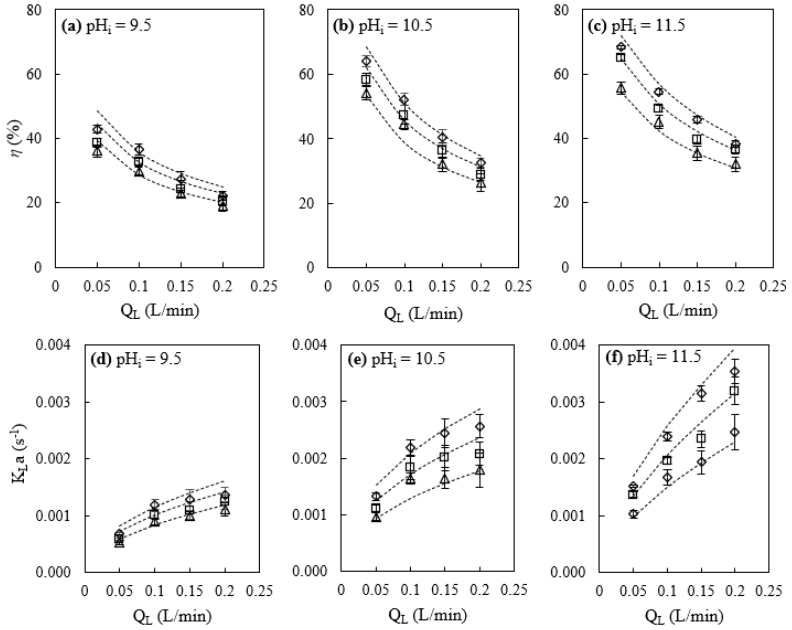
Figure 3.12. Effect of Q_L on \eta and K_{L,a} of NH_3-N stripping from landfill leachate
