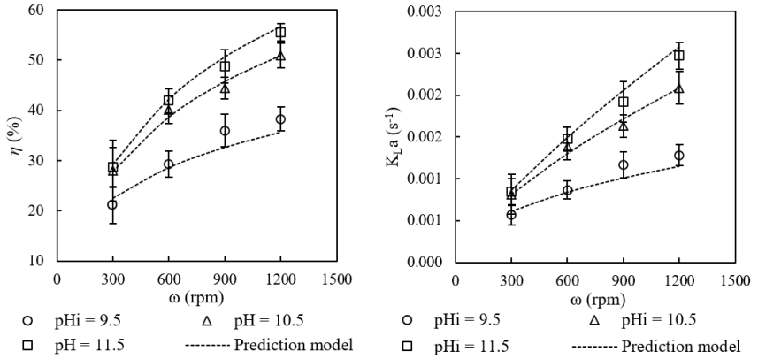
Figure 3.10. Effect of \omega on \eta and K_{La} of \text{NH}_3\text{-N} stripping from landfill leachate
