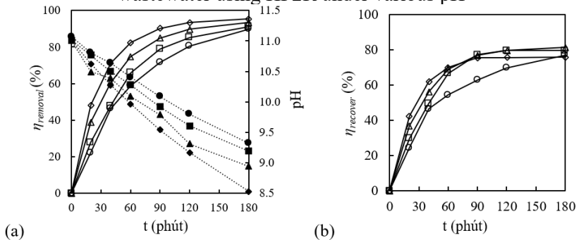
Figure 3.17. Ammonia stripping (a) and recovery (b) from synthetic wastewater using HP2R under various Q_G
