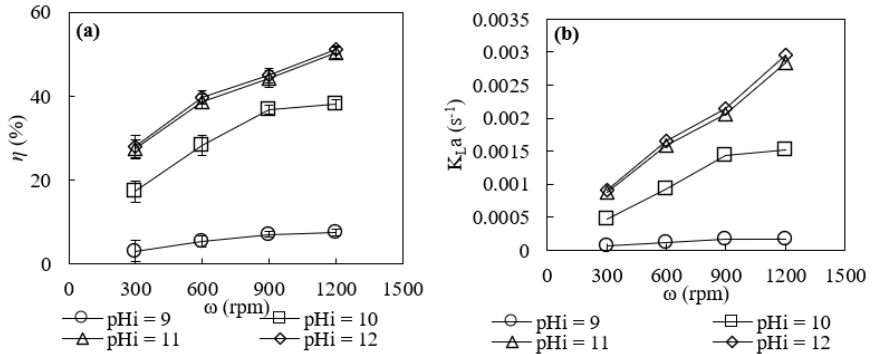
Figure 3.2. Effect of rotational speed on (a) NH 3 -N removal efficiency and (b) K_{L,a}
