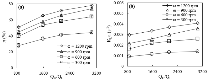
Figure 3.3. Effect of Q_G/Q_L on (a) NH 3 -N removal efficiency and (b) K_{L,a}
