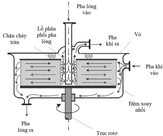
Figure 1.1. Principle of RPB equipment
