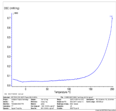
B – DSC thermogram of PHB extracted from S. salina M8 biomass from 200°C to (-30°C)
