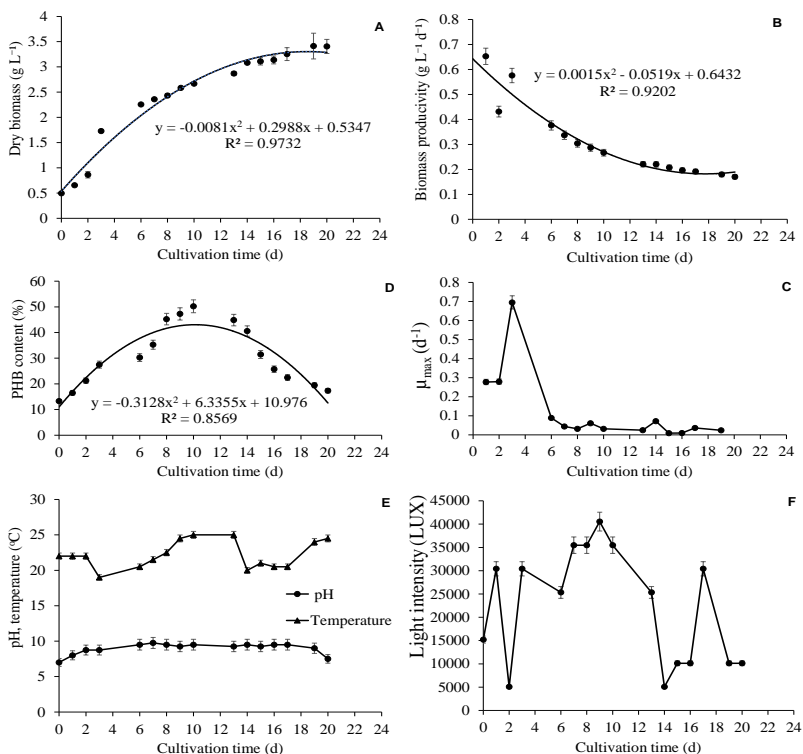
Figure 3.9. Growth performance and PHB accumulation of S. salina M8 cultivated in domestic wastewater using a 30 L vertical tubular photobioreactor
