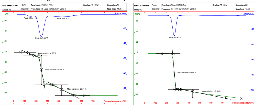
A - TGA/DTG thermograms of PHB extracted from S. salina M8 biomass
