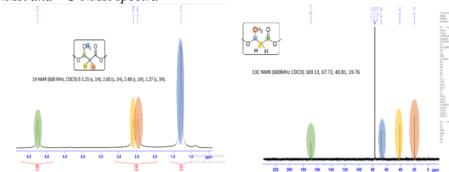
Figure 3.11. ^1\text{H-NMR} (A) and ^{13}\text{C-NMR} (B) spectra of PHB bioplastic
