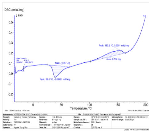
(C) - Second DSC heating scan of PHB extracted from S. salina M8 biomass from -30°C to 200°C
