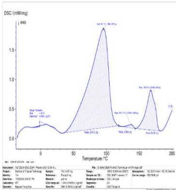
A- DSC thermogram of PHB extracted from S. salina M8 biomass from (-30°C) to 200°C
