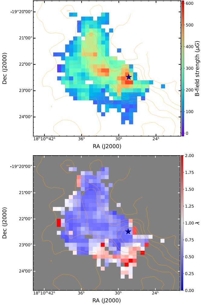
Figure 3.5: Upper: Map of magnetic field strengths calculated for each pixel toward the center region of G11. Lower: Map of mass-to-flux ratio toward the center region of G11. The dark blue star indicates the location of the massive protostellar candidate (P1). The contours are the same as in Figure 3.3.
