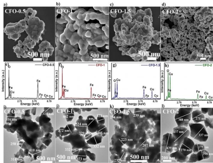
Figure 3.8. Scanning electron microscopy (SEM) images, energy-dispersive X-ray spectroscopy (EDX) spectroscopy, and transmission electron microscopy (TEM) images of the CFO material.
