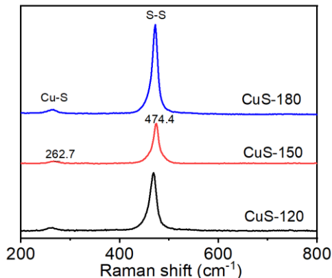
Figure 3.12. Raman spectroscopy of CuS materials synthesized by the solvothermal method at different temperatures (120, 150, 180 °C).
