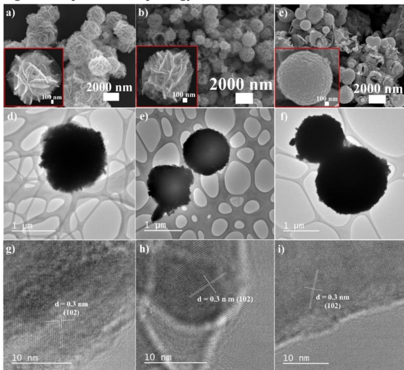
Figure 3.13. SEM, TEM, and HR-TEM images of solvothermal CuS materials prepared at different temperatures: a, d, g) CuS-120; b, e, h) CuS-150; c, f, i) CuS-180.
