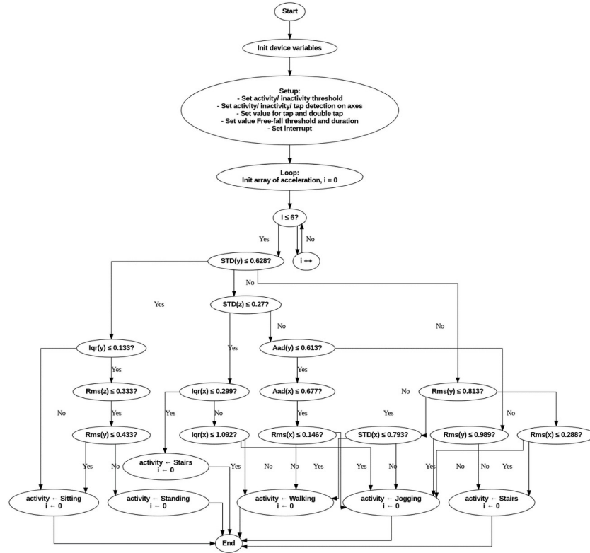
Figure 3.1. Embedded program for real-time activity classification
