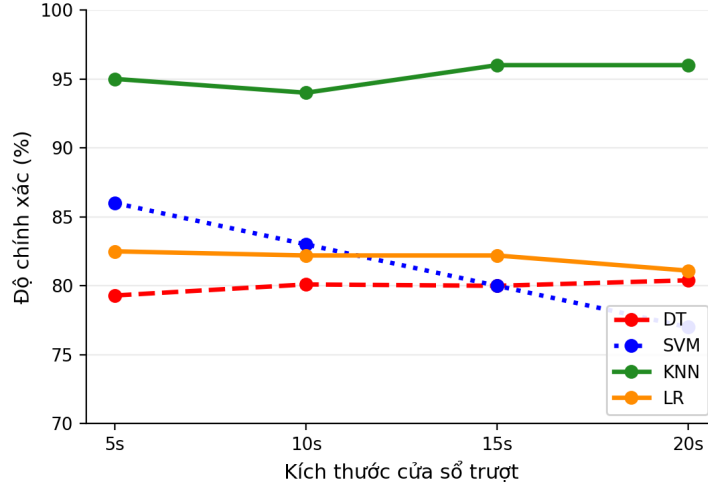
Figure 3.13. Accuracy of DT, SVM, KNN and LR on the public dataset
