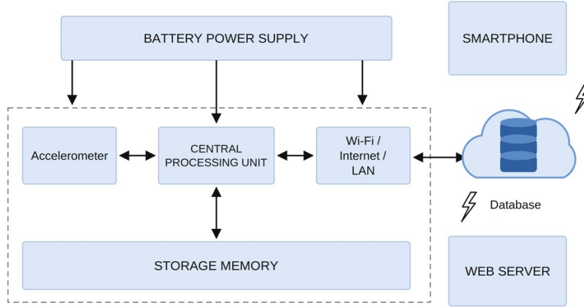
Figure 2.1. Block diagram of the activity classification process
