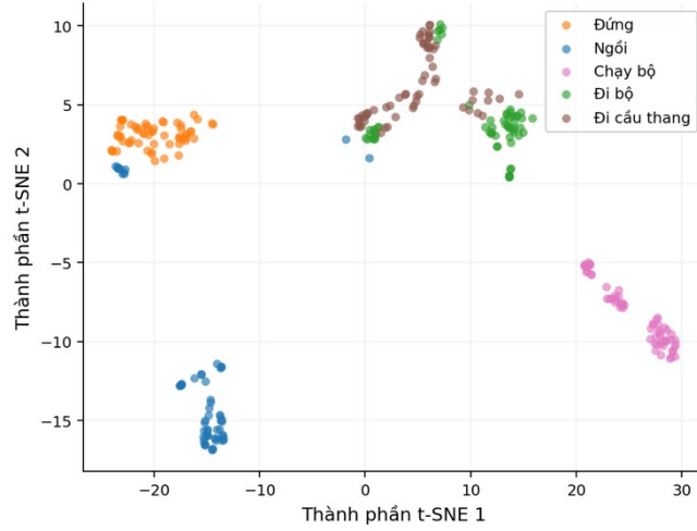
Figure 3.4. WISDM dataset represented in 2D space: (a) without features and (b) with features
