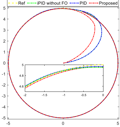
Fig. 3.5. Trajectory tracking in case 1.
