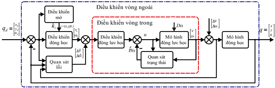
Fig. 3.15. Structure of FB-IFO-SMC-ESO
